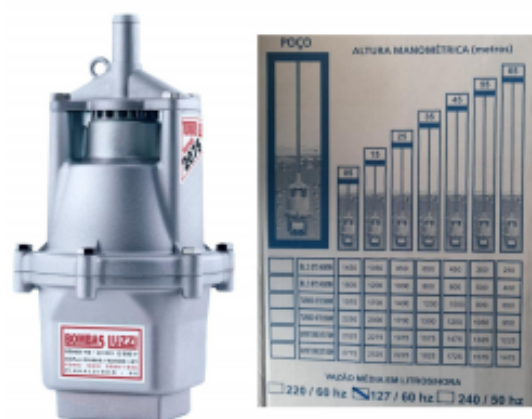
REF: 2093 Bomba Submersa 2075 220V 850W
